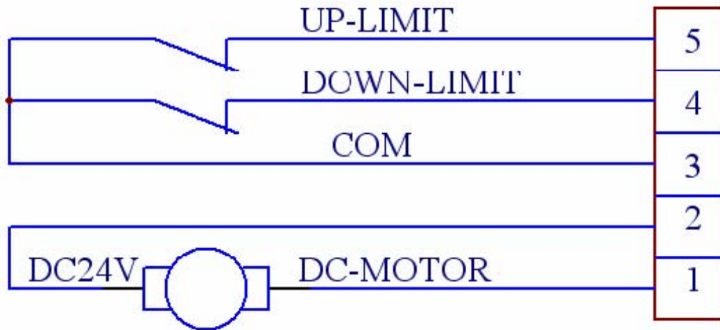
Figure 23: Connection of Down/Up limited and motor
