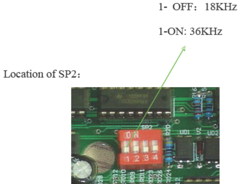
Figure 20: PWM frequency switch
