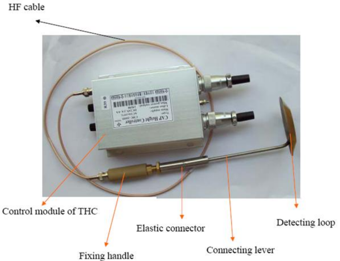
Figure 7: HCB2001 Assembly
