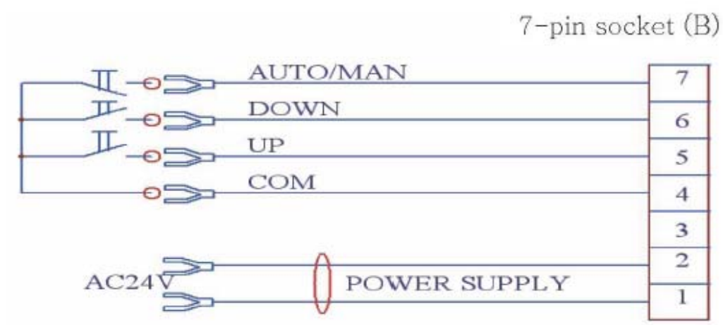
Figure 22: Connection of CNC
