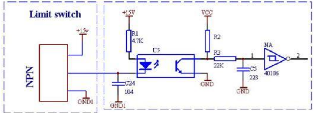
Figure 17: Limit Switch mode.
