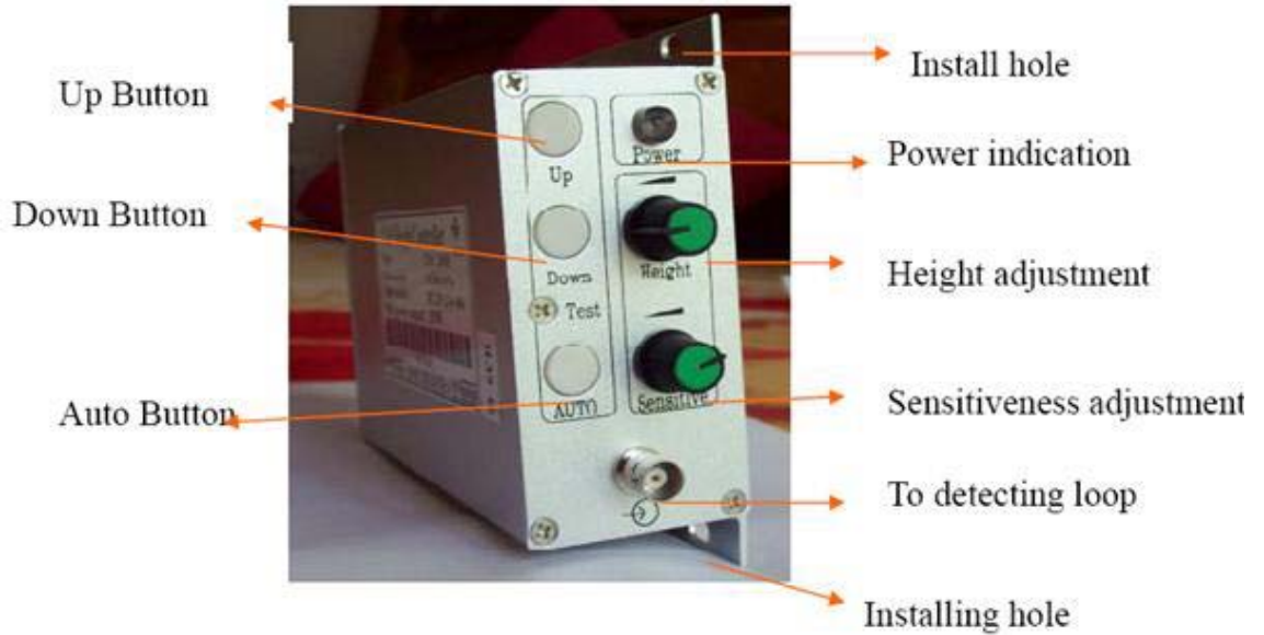
Figure 2: View of operation panel
