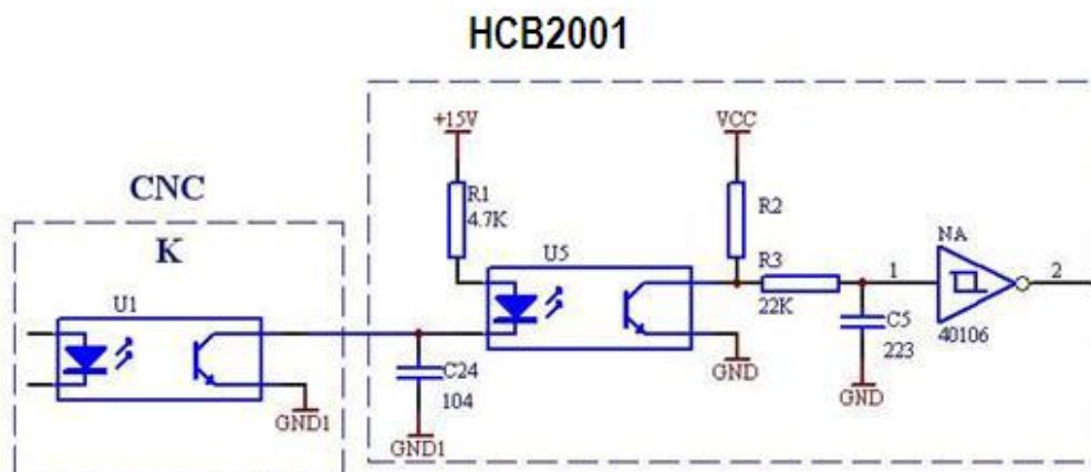
Figure 16: Optical-isolation ↵
